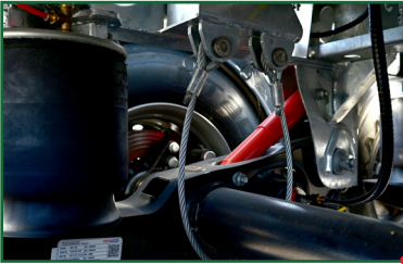
AXLE PROTECTION WHEN LIFTING THE TRAILER
